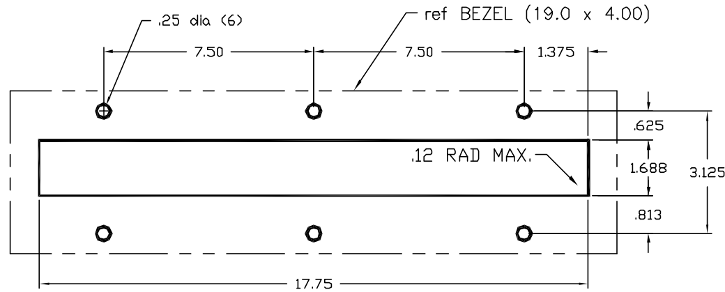
PAPER PATH 17 enclosure cutout
